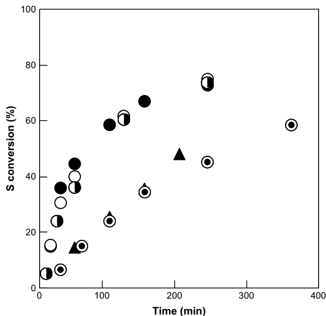
Fig. 1. Conversion–time plots based on S for TEMPO-mediated copolymerization of S and DVB (1 mol%) at 125 °C using DOWFAX 8390 as surfactant under various conditions ( [P(S-r-MA)]_0 = 20 mM): miniemulsion with P(S-r-MA)-TEMPO containing 32 mol% MA (●; d_n \approx 85 nm; d_w \approx 111 nm; ◐; d_n \approx 1000 nm; d_w \approx 1075 nm), 13 mol% MA (◑; d_n \approx 87 nm; d_w \approx 107 nm), PS-TEMPO (0 mol% MA) (○; d_n \approx 65 nm; d_w \approx 79 nm) and bulk (▲; P(S-r-MA)-TEMPO with 32 mol% MA).
