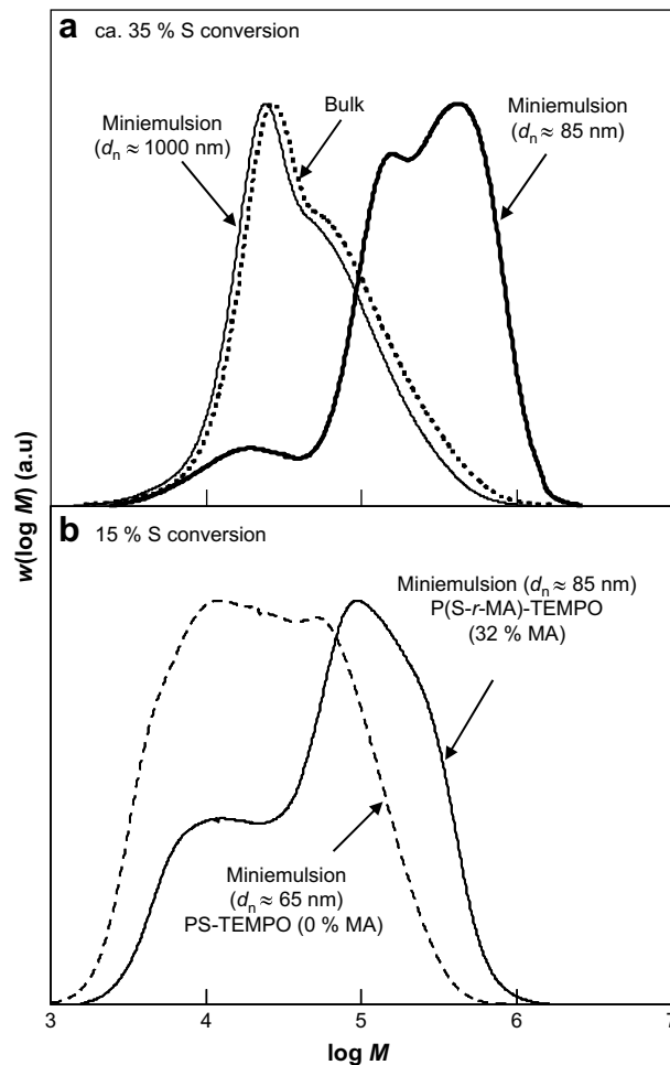
Fig. 4. Molecular weight distributions for TEMPO-mediated copolymerization of S and DVB (1 mol%) at 125 °C using [macroinitiator]_0 = 20 mM in bulk and miniemulsion at similar S conversions. (a) P(S-r-MA)-TEMPO (32 mol% MA) in miniemulsion with d_n \approx 85 nm; d_w \approx 111 nm (thick line; 35% S conversion) and d_n \approx 1000 nm; d_w \approx 1075 nm (thin line; 34% S conversion), and bulk (dotted line; 35% S conversion). (b) Miniemulsion: P(S-r-MA)-TEMPO (32 mol% MA) with d_n \approx 85 nm; d_w \approx 111 nm (full line; 15% S conversion) and PS-TEMPO (0 mol% MA), d_n \approx 65 nm; d_w \approx 79 nm (broken line; 15% S conversion).
