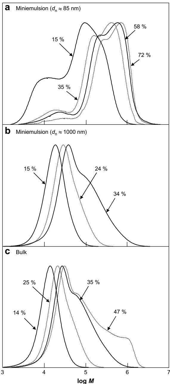
Fig. 3. Molecular weight distributions normalized to peak height for TEMPO-mediated copolymerization of S and DVB (1 mol%) using DOWFAX 8390 as surfactant at 125 °C ( [P(S-r-MA)-TEMPO]_0 = 20 mM; 32 mol% MA macroinitiator) in (a) miniemulsion ( d_n \approx 85 nm; d_w \approx 111 nm); (b) miniemulsion ( d_n \approx 1000 nm; d_w \approx 1075 nm) and (c) bulk.
